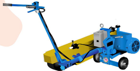
Reciprocating Grinder Semi-automatic and programmable.
